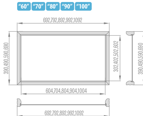
Top lights for fixed door frame in single leaf doors
