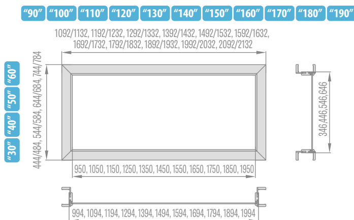
Top lights for adjustable door frame in double-leaf doors strip 6cm /strip 8cm
