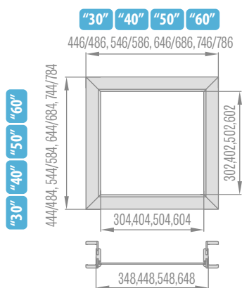
Top lights for adjustable door frame in double-leaf doors strip 6cm /strip 8cm
